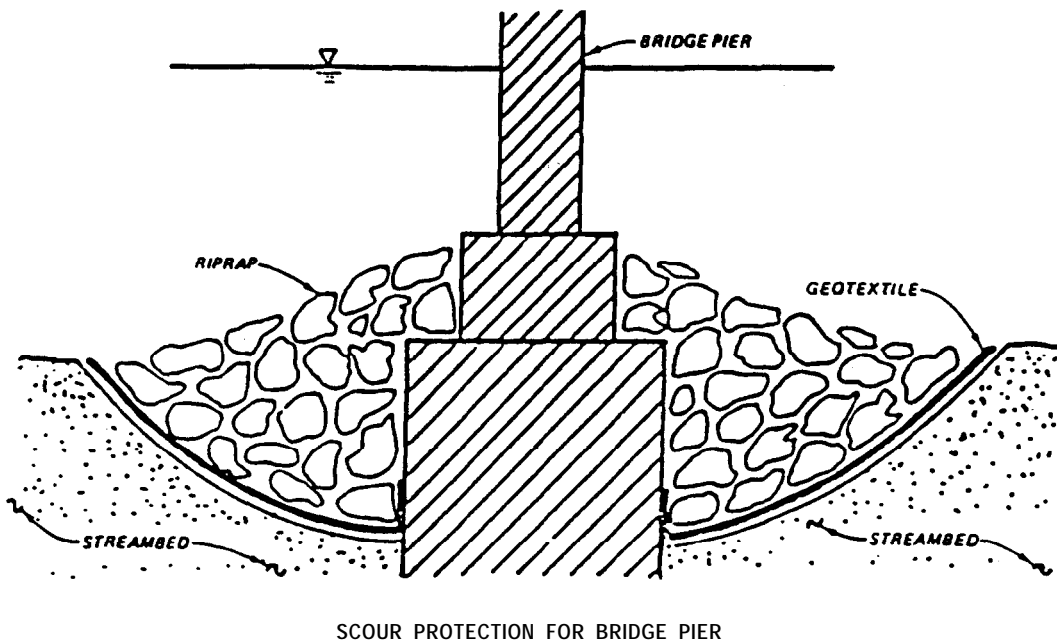
Figure 6-6. Use of Geotextiles around Piers and Abutments.
